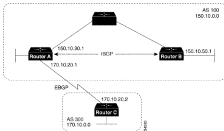
Figure 12-13: Next Hop Attribute
