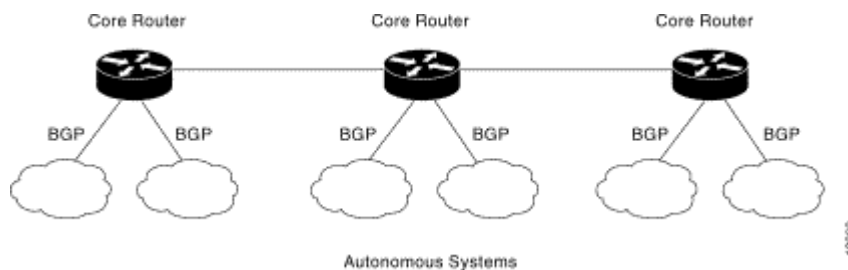
Figure 35-1: Core routers can use BGP to route traffic between autonomous systems.
