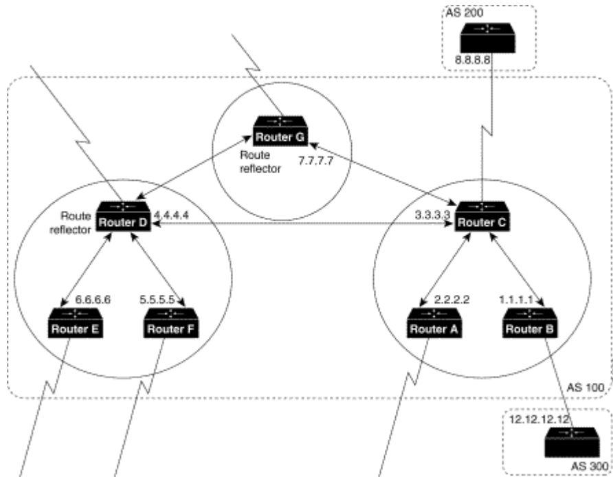
In Figure 12-30 , Routers A, B, and C form a cluster, and Router C is the route reflector. Routers D, E, and F form a second cluster, of which Router D is the route reflector. Router G forms a third cluster. Note that Routers C, D, and G are fully meshed and that the routers within a cluster are not fully meshed.
