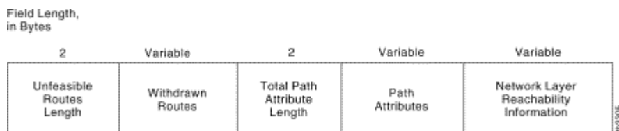
Figure 35-5: A BGP update message contains five fields.
